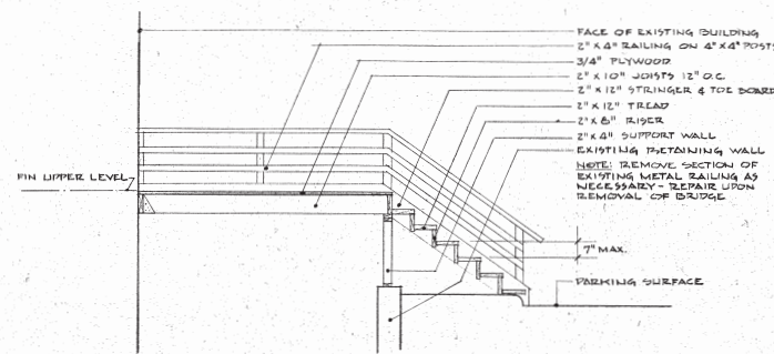
SECTION THRU TEMPORARY BRIDGE SCALE: 3/8" = 1'-0"
