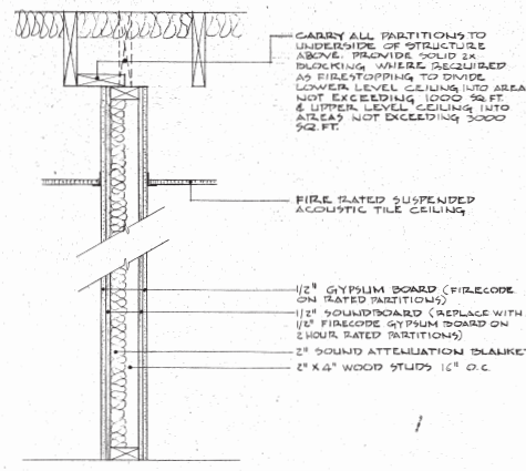
TYPICAL INTERIOR PARTITION SCALE: 1 1/2" = 1'-0"
